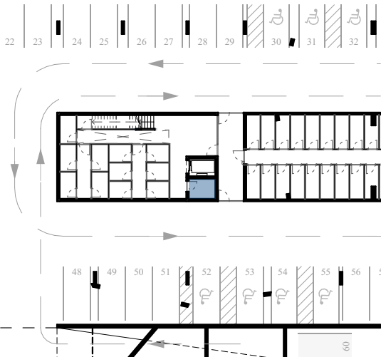
Položaj shrambe - S 26, klet -2, M 1_500
