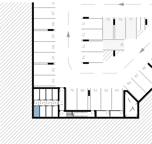
Položaj shrambe - S 68, klet -2, M 1_500
